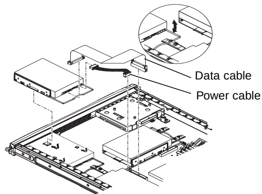
Figure 1-2 Installing a Hard Disk Drive (Sun Fire V100 shown)
